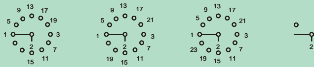
ST 101/... ST 111/... ST 121/... STO 11/...
