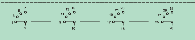
ST 44/... 4 Position 4 Pole Selector Switch
