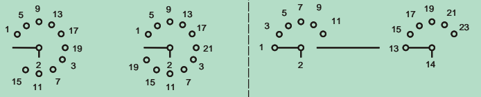
STO 101/... STO 111/... ST 62/... 6 Position 2 Pole Sw.
