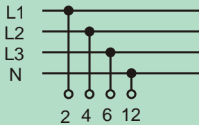
Voltmeter Selector, Phase to Phase & Neutral V 30/....
