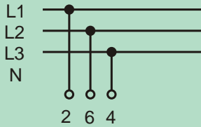
Voltmeter Selector, Phase to Phase & Neutral V 13/....
