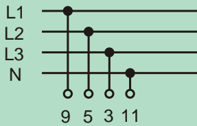
Voltmeter Selector, Phase to Phase & Neutral V 31/....
