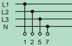
Voltmeter Selector, Phase to Neutral V 3/....
