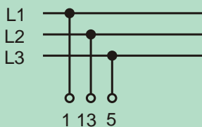
Voltmeter Selector, Phase to Phase, Two Supplies V 32/....
