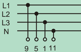
Voltmeter Selector, Phase to Phase & Neutral VN 30/....
