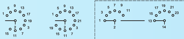
STO 101/... STO 111/... ST 62/... 6 Position 2 Pole Sw.
